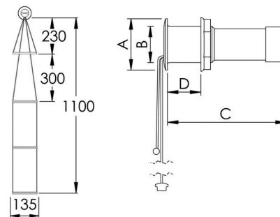
3 Step Emergency Ladder + Holder
