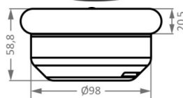
Discovery LED All Round White Navigation Light
