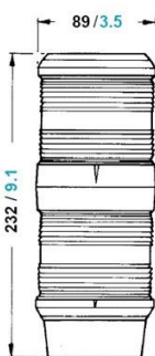
Tri-colour Anchor Standard Fit - 2nm
