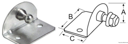
Gas Strut 90° plate Ø 10mm-ball internal
