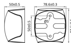
Sphera II LED Stern Navigation Light
