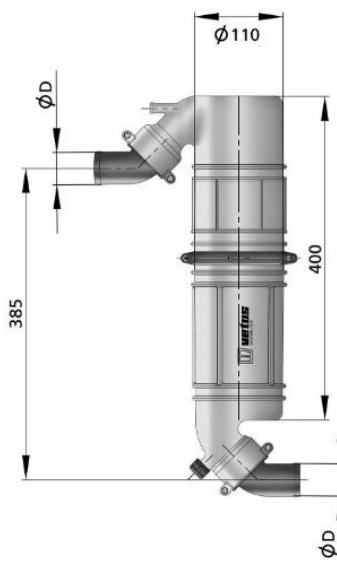
NLPG40, 45, 50. 3 litres capacity
