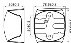
Sphera II LED Bow Navigation Light
