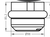
Discovery LED Tri-Colour + Anchor Navigation Light
