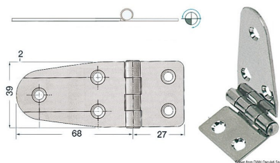
Stainless Steel Hinge
