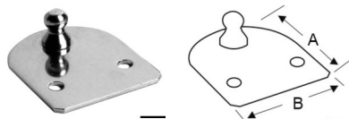
Flat Fastening Plate Ø 10mm-ball
