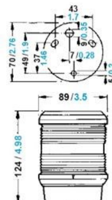
All Round White Light - 2nm
