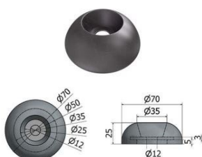
70mm Metec 0.4kg Disc Anode (MD4Z)
