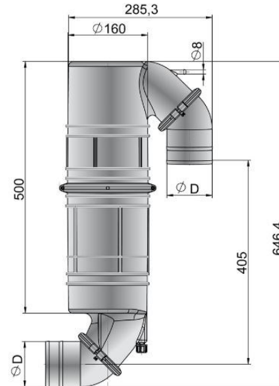
NLPG60, 75, 90. 10 litres capacity
