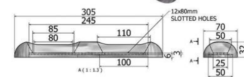
305mm Metec 2.8kg Bolt On Hull Anode (MH28ZS-2)
