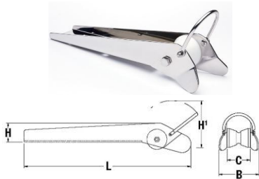
Maxwell Fixed Bow Roller (ARWU-04)
