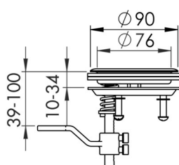
Compression Lift and turn flush latch External Ø 90mm
