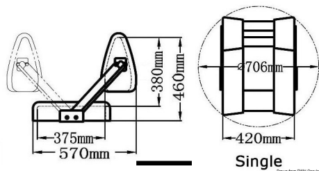
Reverso White Single Seat + Rotating Backrest RAL 9010
