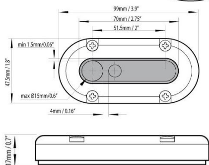
Aluminium Cable Gland.
