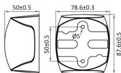
Sphera II LED Port Navigation Light
