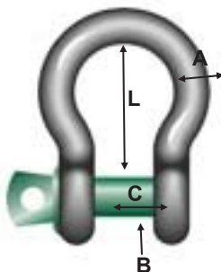
Tested Green Pin Bow Shackles
