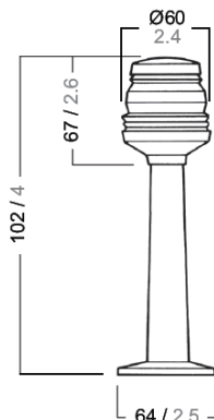
All Round White Anchor Pedestal Mount Light - 2nm
