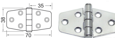
Stainless Steel Backflap Hinges (Sold Each)
