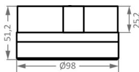
Discovery LED Bi-Colour Navigation Light
