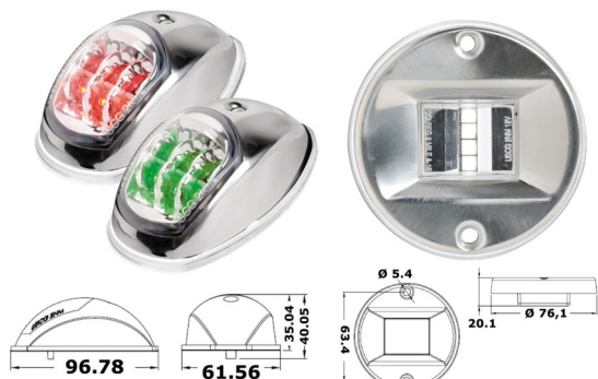
Port & Starboard SS LED Light
