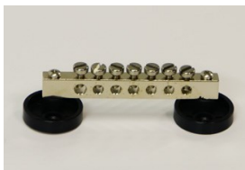
F-2241 6 Way Screw Terminal 1 x 5mm hole + 6 x 4mm holes. Current rating: 100A
