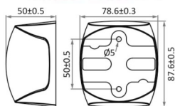
Sphera II LED Starboard Navigation Light
