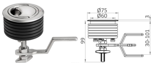
Eclipse MK2 75mm Flush Latch
