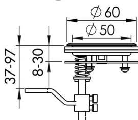
Compression Lift and turn flush latch External Ø 60mm
